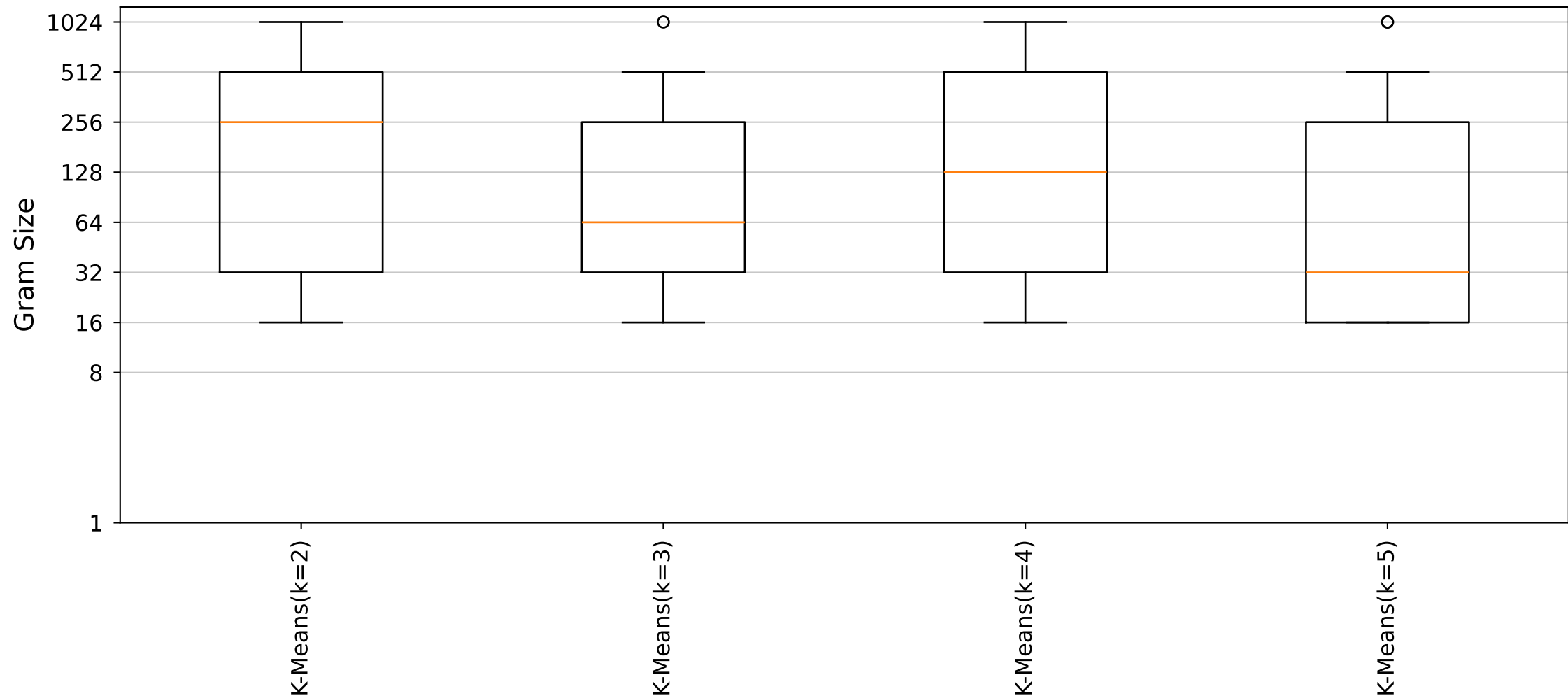
YARA Rules Gram Size Distribution (Cluster45_Size5 dataset)
